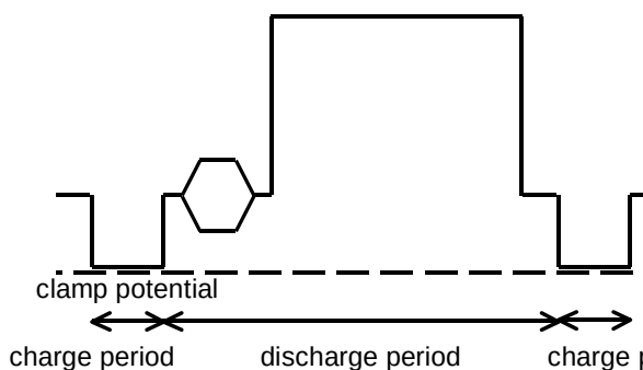
< Waveform of input terminal >
