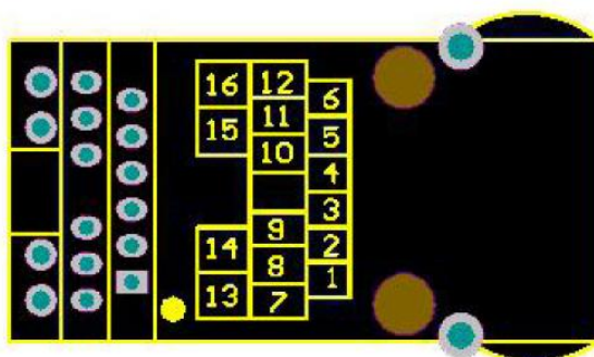
Figure 2. Eport Pro-EP10 管脚定义
