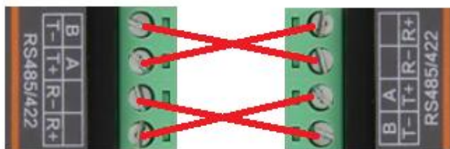
Figure 5. HF5111A RS422接线图
