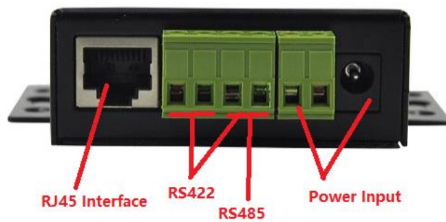
Figure 3. HF5111A 侧面图
