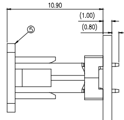
CAP ASSEMBLY AND MOUNTING CONDITION (REF)
