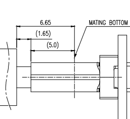
MATED CONDITION (REF)
