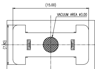
CAP ASSEMBLY AND MOUNTING CONDITION (REF)
