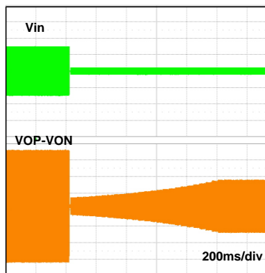
NCN release time
