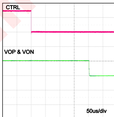
Class_AB shutdown time
