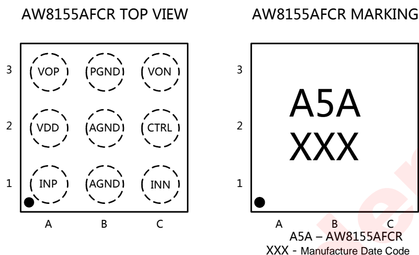
Figure 1. Pin Configuration and Top Mark of AW8155A
