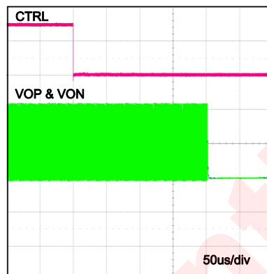
Class_D shutdown time
